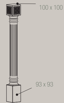
GAMBA ISOLA C/DECORO LEG FOR PENINSULA "H" = 870
